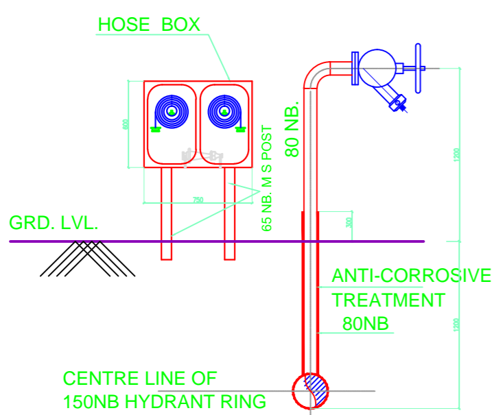
TYP. MOUNTING DETAIL OF YARD HYDRANT ON UNDER GROUND PIPING
