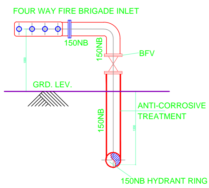
DETAIL OF FOUR WAY FIRE BRIGADE INLET CONNECTION FOR U/GROUND TANK FILLING
