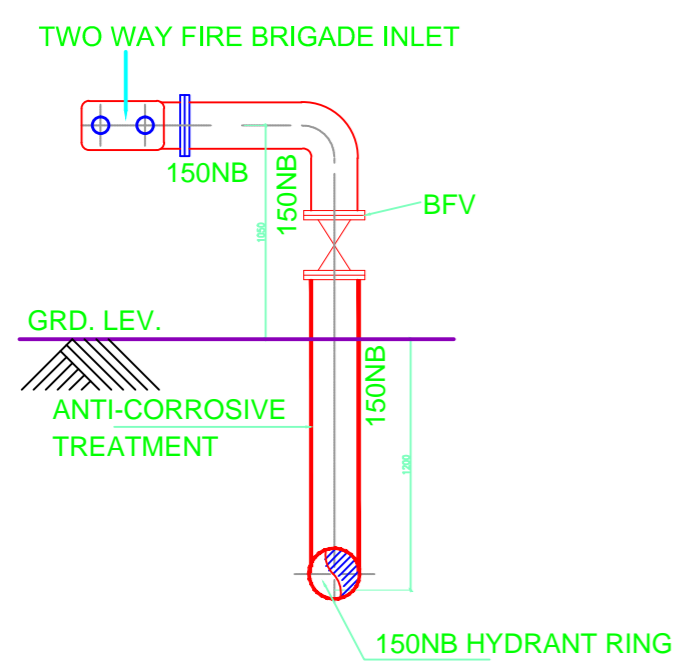
DETAIL OF TWO WAY FIRE BRIGADE INLET CONNECTION
